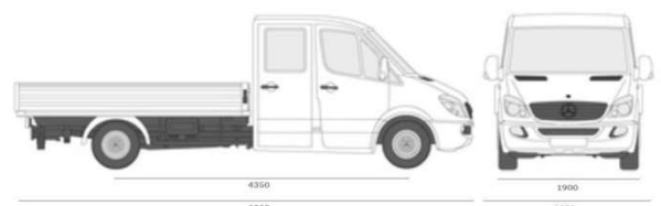
Typical 5t LGV Site Pickup
