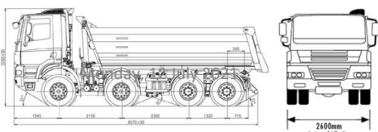
Typical 40t HGV for Granular Materials
